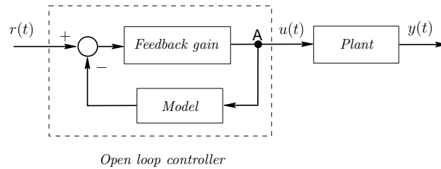
Figure 2.9: Open loop controller
