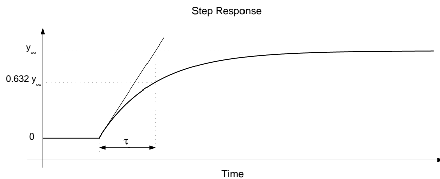
Figure 4.4: Step response of a first order system
