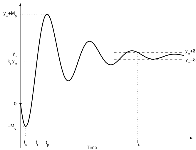
Figure 4.3: Step response indicators
