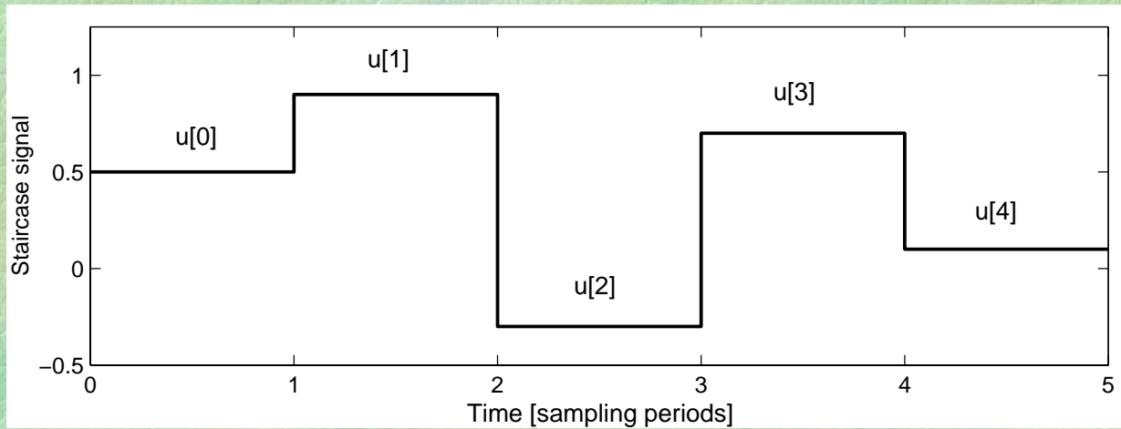
Figure 12.2: Staircase reconstruction
