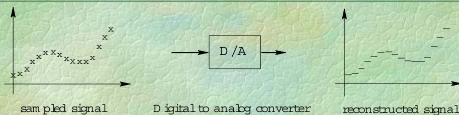
Figure 12.11: The result of reconstruction
