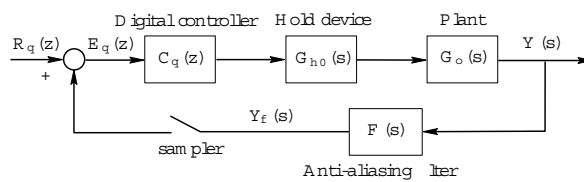
Figure 13.1: Sampled data control loop
