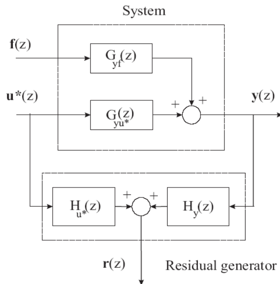
Figure 2.10: Residual generator general structure. 11/10/2007
