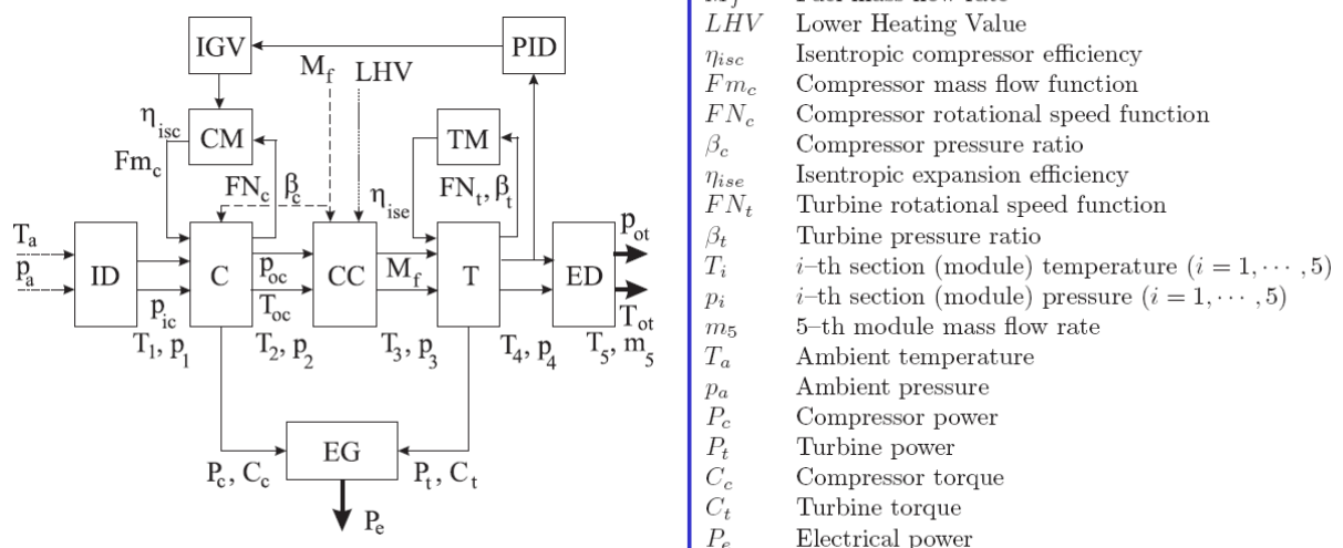
Figure 5.2: Block diagram of the single-shaft gas turbine.
