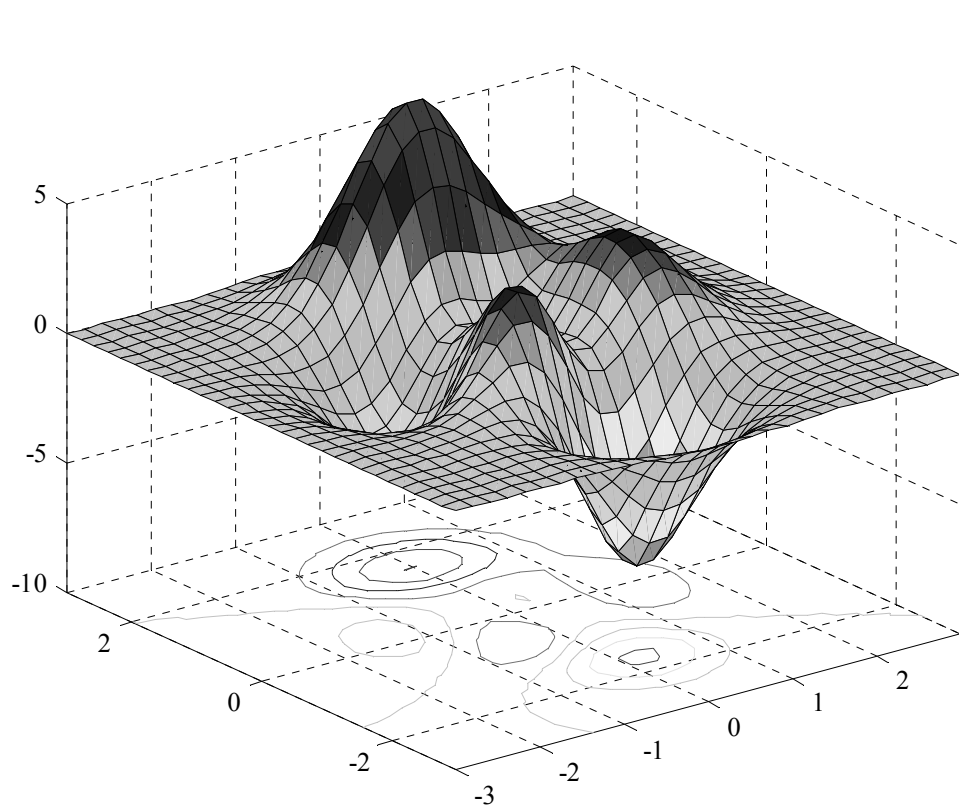
2 dimensional Gaussian
